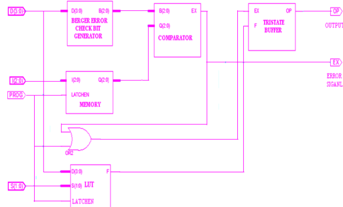
Figure 2: Block Diagram of Look Up Table With Berger Checker Circuit
