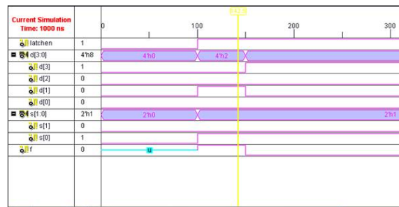
Figure 4: Simulation output for LUT
