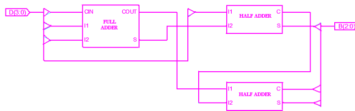
Figure 3: Block Diagram of Berger Error Check Bit Generator
