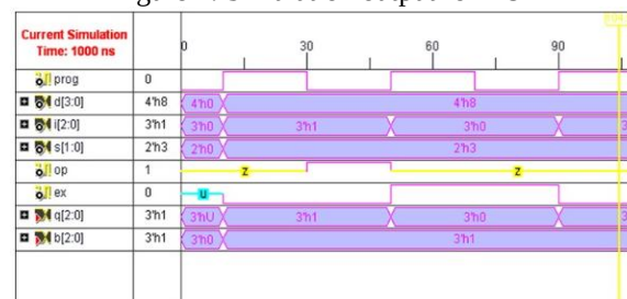
Figure 5: Simulation output for LUT with Berger combinational checker circuit
