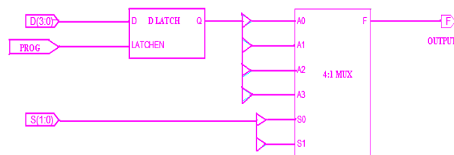
Figure 1: Block Diagram of LUT
