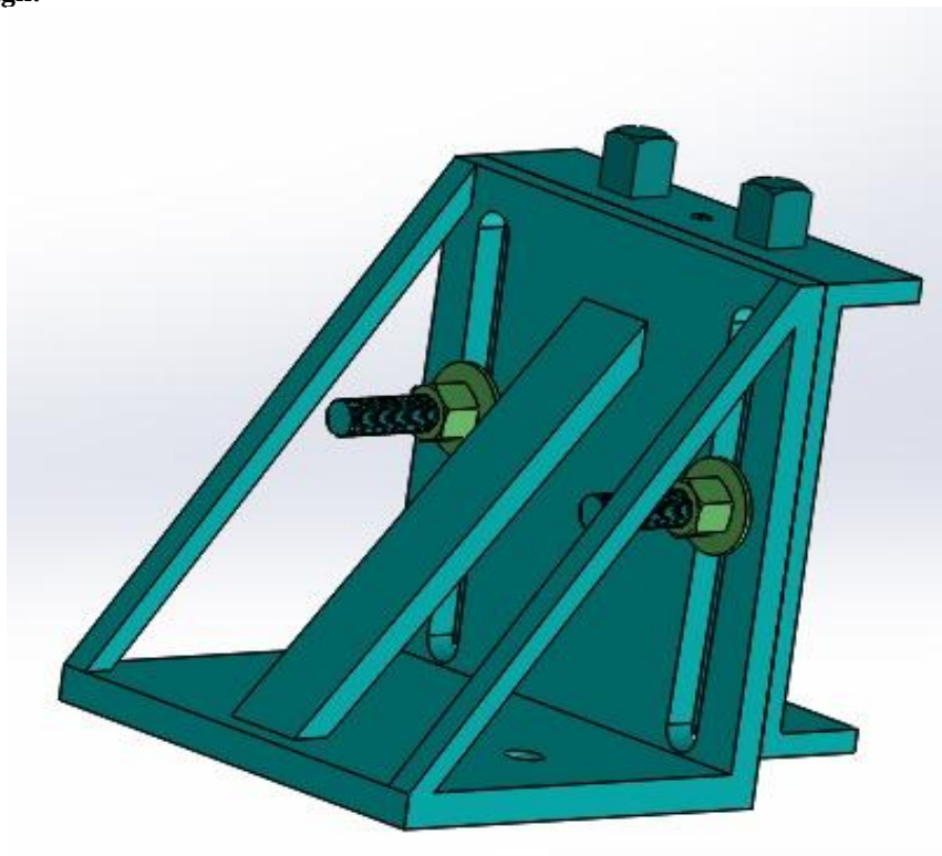
Figure 7: 3D View of Fixture Design
