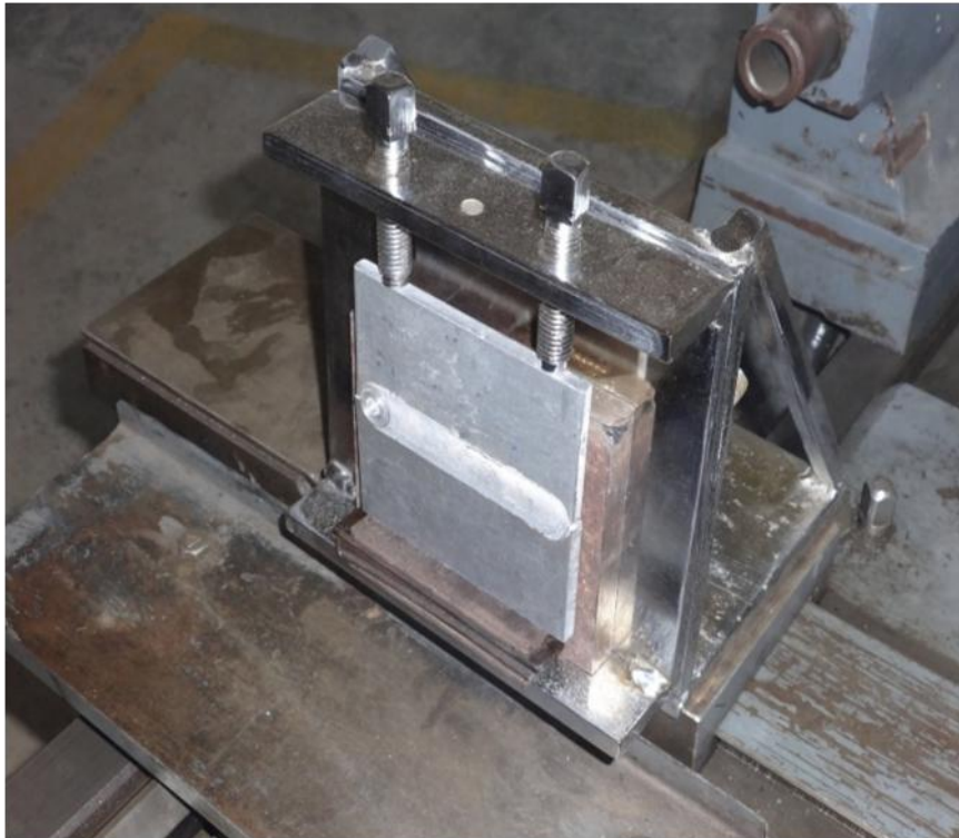
Figure 10: Welding Fixture Design
