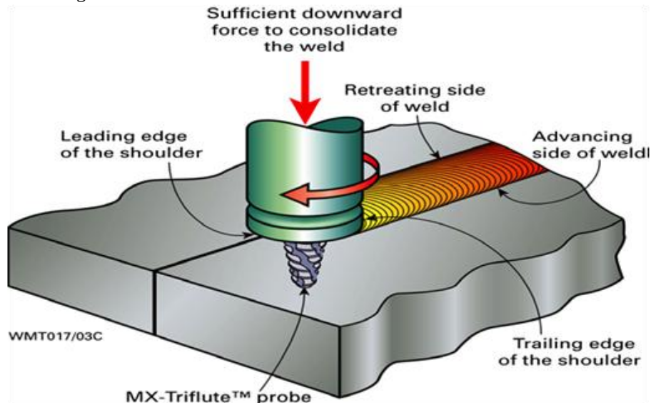
Figure 8: Friction Stir Welding Process
